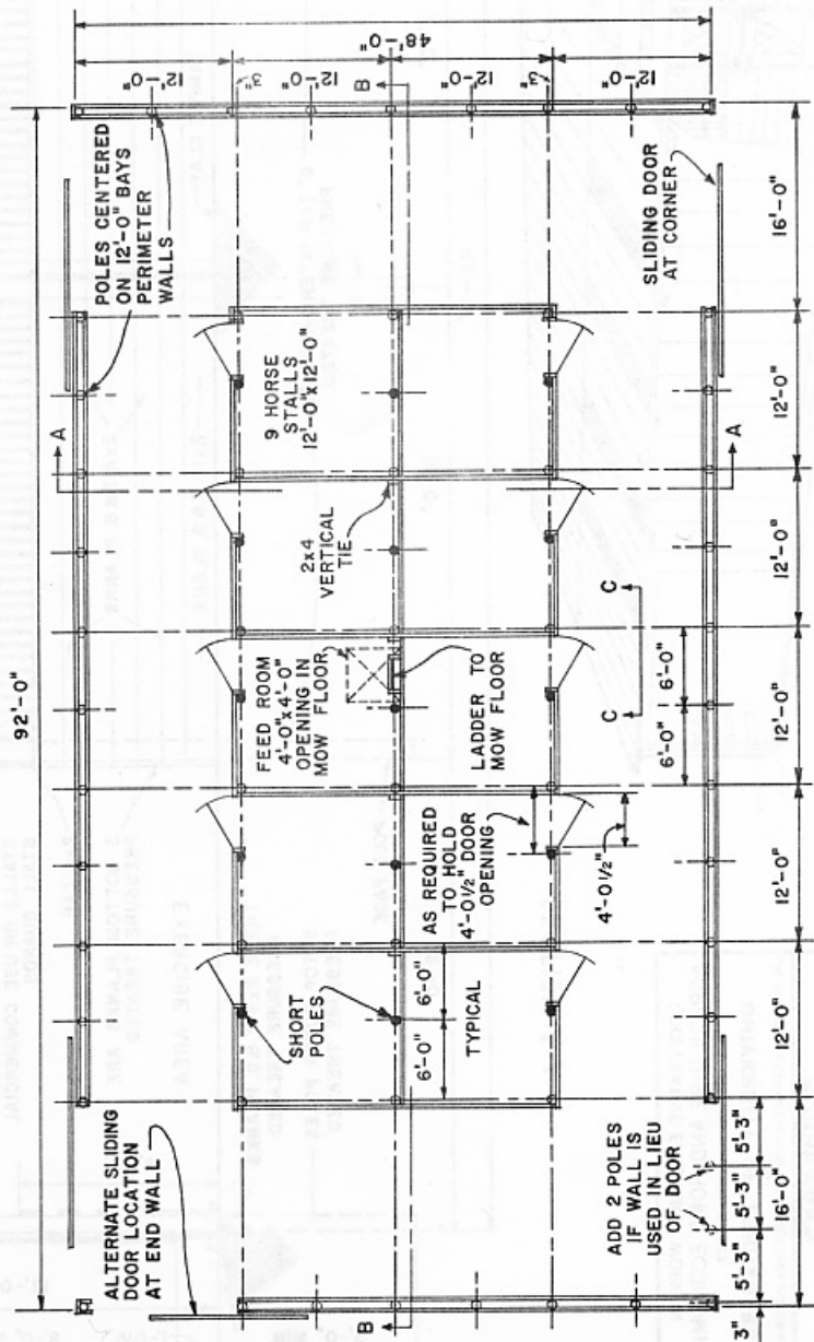
FLOOR PLAN
