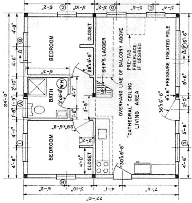
PLAN 0 2 4 6 FT.
