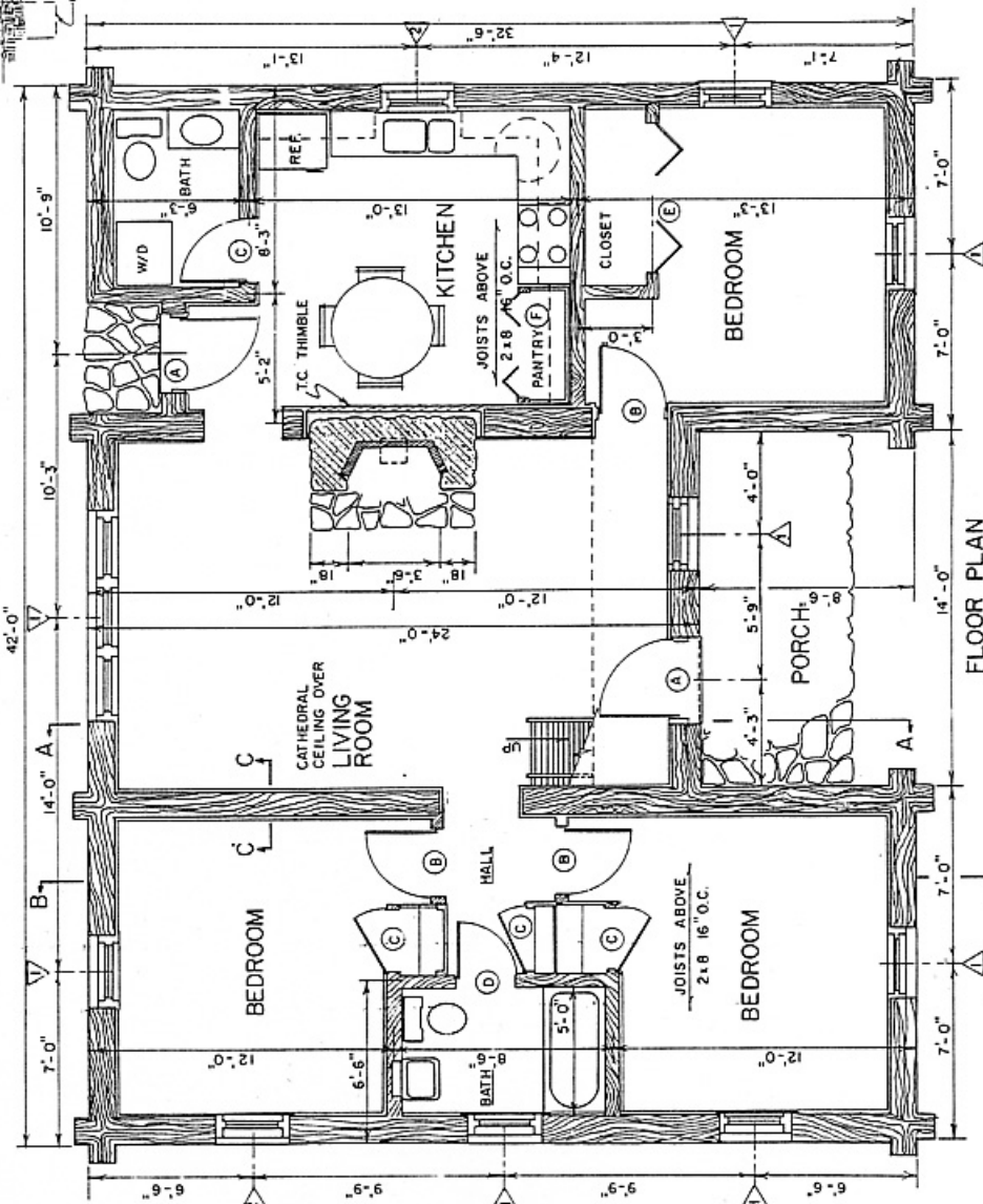
SECOND FLOOR PLAN NO SCALE
